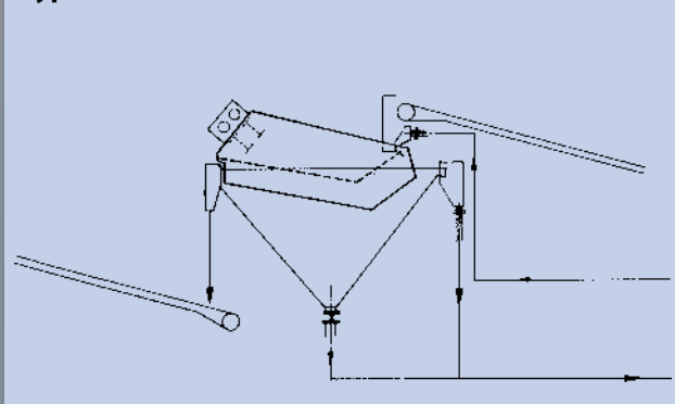
Typical flow-sheet
